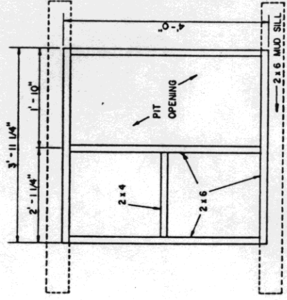
BASE FRAMING PLAN (NO SCALE)
