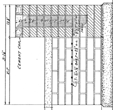
SECTION
