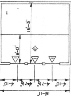
LOFT DETAIL
