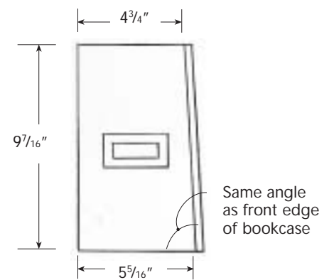
RIGHT-SIDE JIG
