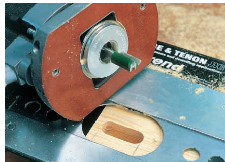
The rounded ends of the mortice perfectly match those of the tenon.
