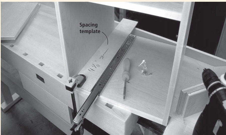
A spacing template makes getting the drawer slides mounted to the cabinet easier and helps ensure that you won't need to do as much adjusting to fit the drawers.
