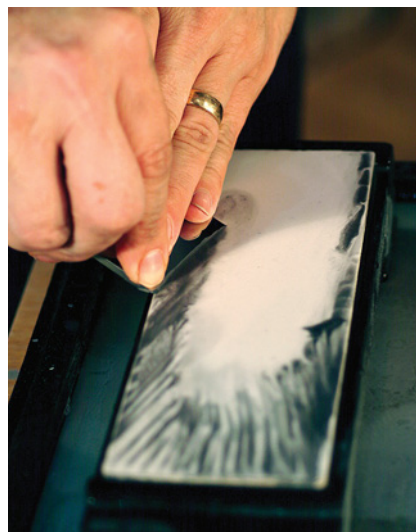
As you prepare to sharpen the bevel, the right hand is again loosely holding the blade, providing light support with the bevel flat against the stone. Seat the bevel on the stone. Your right hand is only supporting and balancing the iron; the index finger applies light pressure to hold the bevel flat on the stone.
