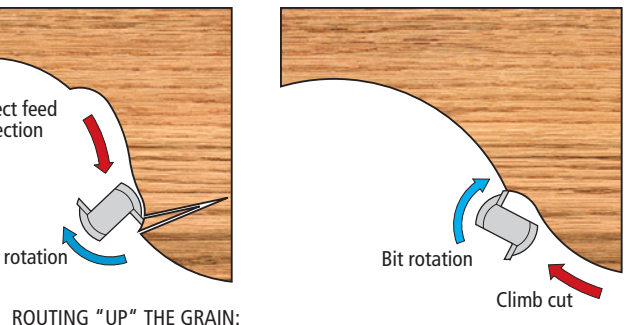
CLIMBING THE UPHILL SECTIONS: Cutting edges sweep down and in on wood fibers
