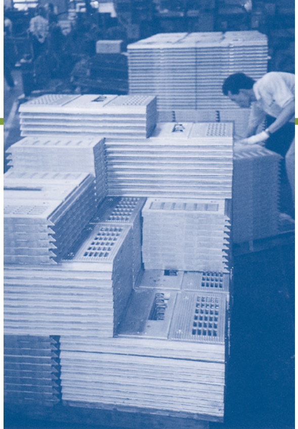
At Hsum Tsao, a Taichung aluminum die cast molding plant, a worker knocks off excess aluminum from a miter saw fence casting (left). Castings for benchtop saws are stacked for machining and assembly later (right).
