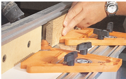
Finger boards make this router-table process safer and ensures an even cut all along the miter.
