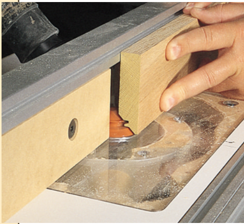
Set up the router table by running a piece on edge over the knife. The cut should leave the interlocking tongue and groove in the center of the miter.
