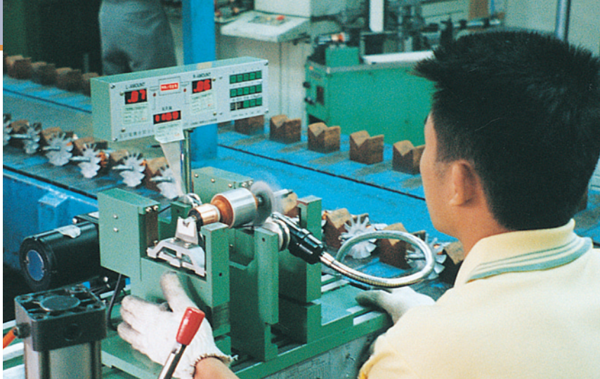
An employee at the Kosta Plant in Taiwan balances the armature on a universal motor. The plant assembles tools and tests motors for Delta Manufacturing.
