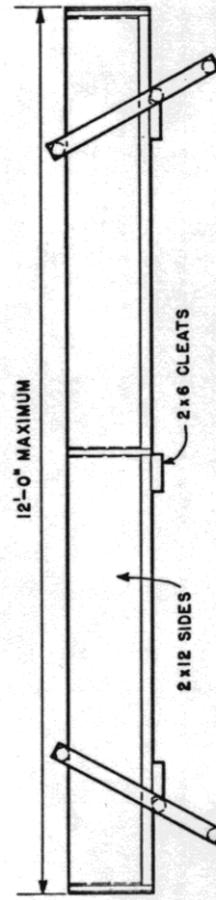
SIDE ELEVATION
