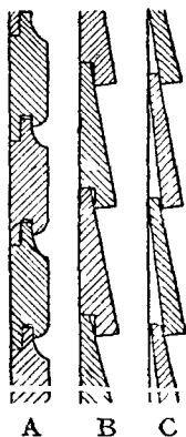
Fig. 343. Weather Boards.
