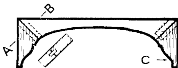
Fig. 107.—Shaped Spandrel for Recess.
