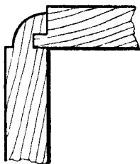
Fig. 118 —Corner Joint with Corner Mould.
