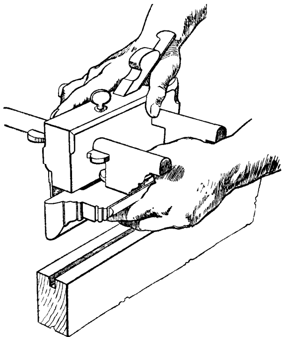
Fig. 122.—Method of using the Plough Plane.
