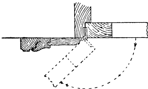
Fig. 247.—Open Joint Hingeing.
