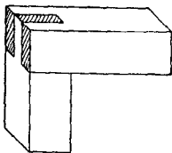
Fig. 78.—Bridle Joint at Corner of Frame.
