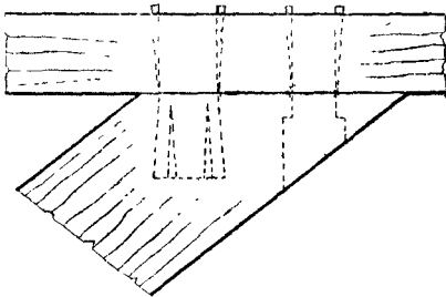
Fig. 174.—Inserted Tenons.
