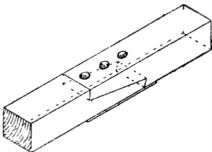
Fig. 213.—Plated Scarf Joint Used in Roof Work.
