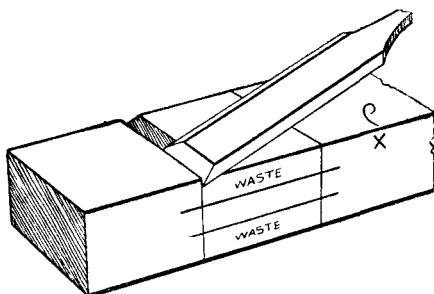
Fig. 88.—Chiselling Operation.
