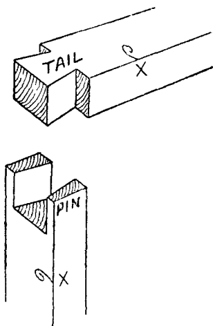
Fig. 300.—Corner Dovetail.
