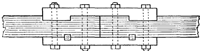
Fig. 217.—Fished Joint.
