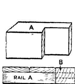
Fig. 127.—Barefaced Tenon Joint.
