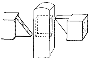
Fig. 144.—Joint for Fencing.
