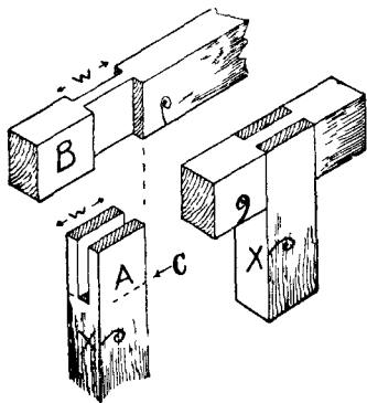
Fig. 81.—Bridle Joint, open and closed.
