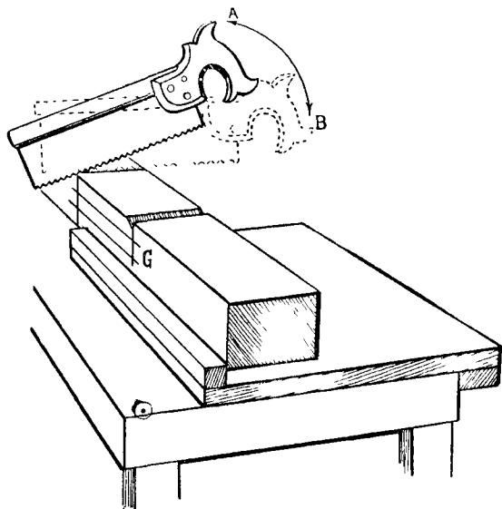
Fig. 89.—Sawing the Shoulders.
