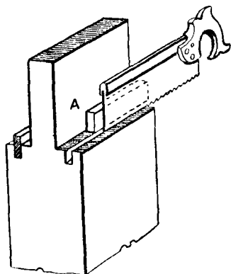
Fig. 126.—Tonguing Shoulders of Tenons.
