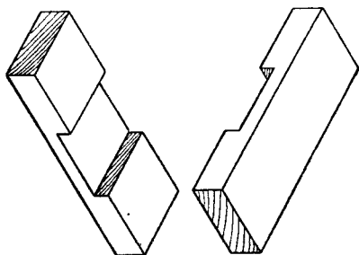
Fig. 39.—Cross Halving Joint.
