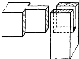
Fig. 169.—The Open-slot Mortise Joint.
