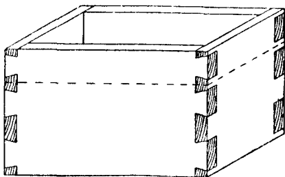
Fig. 299.—Dovetailing for Small Box.
