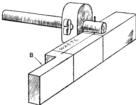
Fig. 65.—Using the Marking Gauge.
