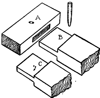
Fig. 162.—Draw-bore Pinning.
