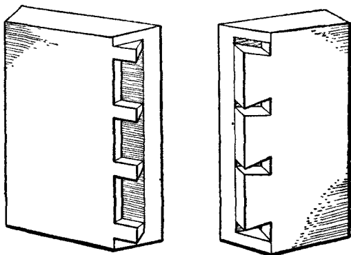
Fig. 288.—Secret Mitre Dovetailing.
