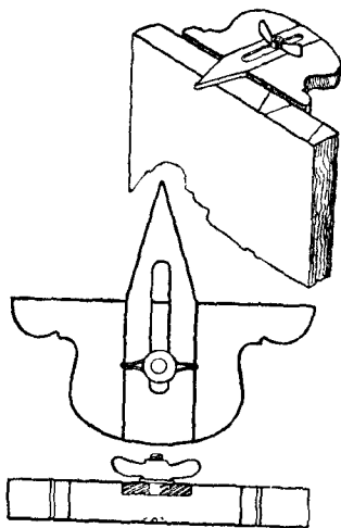
Fig. 304.—Hand-made Template for Marking Dovetails.
