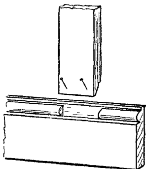
Fig. 347.—Fixing Muntin to Skirting.
