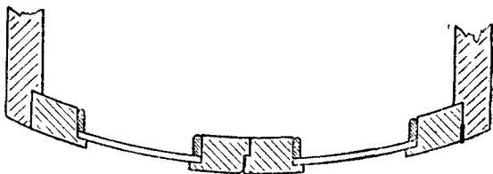
Fig. 260.—Curved Cupboard Doors with Rebated Meeting Joint.
