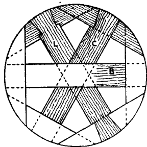
Fig. 45.—Halved Joints on Barrow Wheels.
