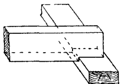
Fig. 352.—End Notch.
