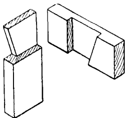
Fig. 35.—Halved Joint with one side Dovetailed.
