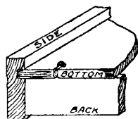
Fig. 368.—Drawer Bottom Joint.
