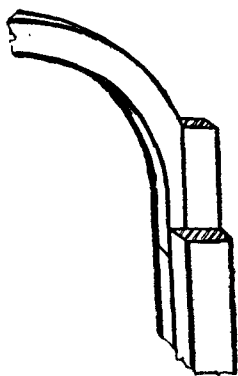
Fig. 339. Method of Building up Semicircular Head of Door Frame.
