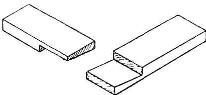
Fig. 36.—Halved Joint with Double Dovetail.
