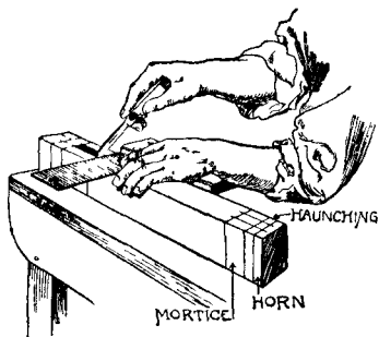
Fig. 178.—Setting Out the Stiles with Marking Knife.
