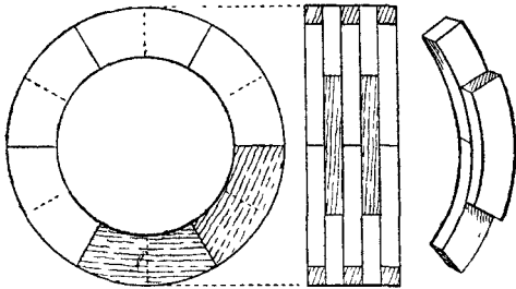
Fig. 23.—Example of Circular Laminated work.
