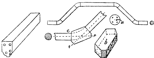
Fig. 200.—Method of Dowelling Thick Timber.
