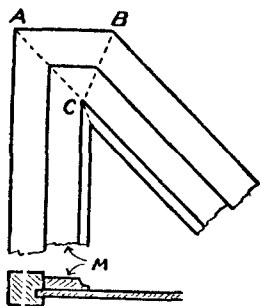
Fig. 330.—Wide Mitred Moulding.
