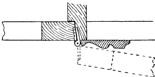
Fig. 249.—Close Joint Hingeing.
