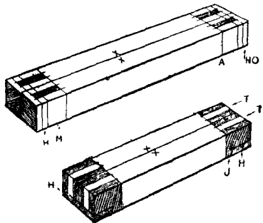
Fig. 177.—Setting out Stiles and Rails for Tenoning.
