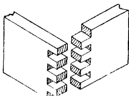
Fig. 111.—Combing or Locking Joint.
