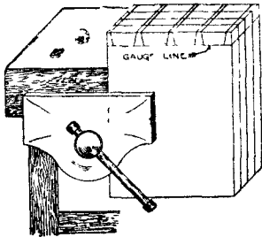
Fig. 283.—Cutting several Dovetails at once.
