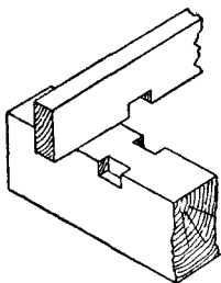
Fig. 353.—Cogged Joint
