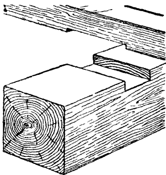
Fig. 350.—Notched Joint.
