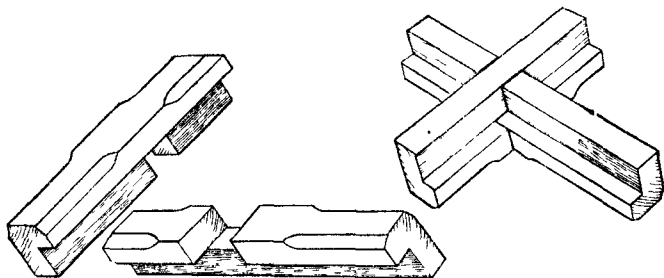
Fig. 61 (B):—Halved Joint of Oxford. Fig. 61 (C).—Back Frame with front edges chamfered. view of Oxford Frame.
