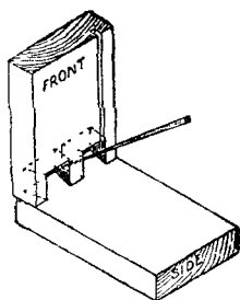
Fig. 278.—Marking Pins on Drawer Side.
