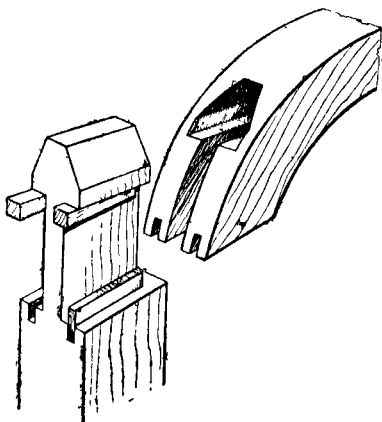
Fig. 171.—Hammer-Head Tenon Joint.
