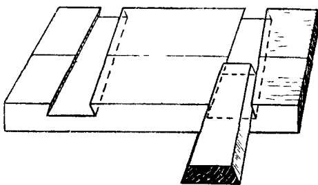
Fig. 289.—Dovetailed Keys for Wide Surfaces.
