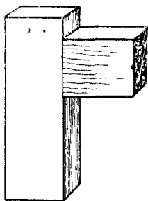
Fig. 137. — Stile and Cross Rail with Horn.
