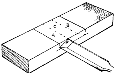
Fig. 68.—Paring away Waste with Chisel.
