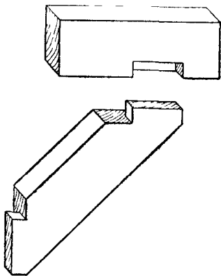
Fig. 31.—Oblique Halving with Shoulder.
