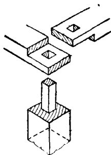
Fig. 151.—Joining Top Rails to Upright Post.
