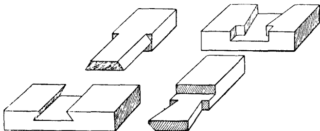
Fig. 43.—Dovetailed and Halved Joint.
