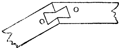
Fig. 291.—Dovetail Keying on the Angle.
