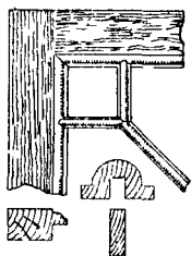
Fig. 110.—Corner of Barred Door.
