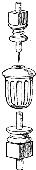
Fig. 349. Method of Building up Turnings.
