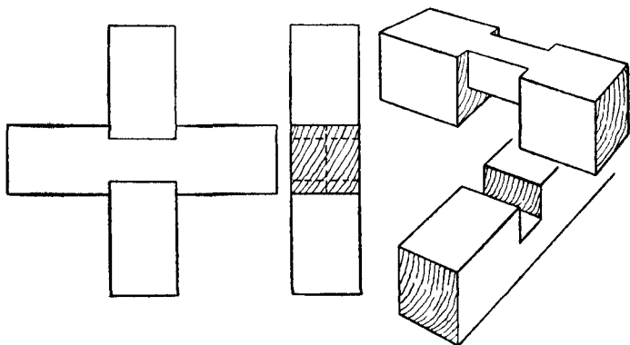
Fig. 55.—Cross Halving Joint with Housed Corners. Fig. 56.—The parts of Fig. 55 shown separate.
