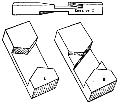
Fig. 46.—Detail of Halved Joints in Fig. 45.
