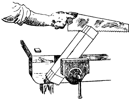
Fig. 180. —Second Operation in Sawing Tenons.
