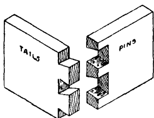
Fig. 269.—Dovetails for Boxes, etc.
