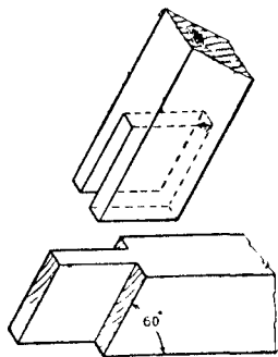
Fig. 170.—Open-Slot Mortise at 60 degrees.
