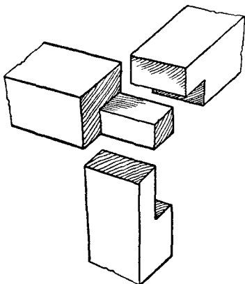
Fig. 57.—Cross Rail and Upright Halved Joint.
