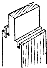
Fig. 166.—Tenon with Tongued and Grooved Shoulder.
