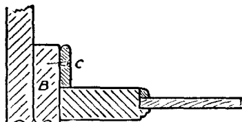
Fig. 254.—Showing Cupboard End Thickened (see B).
