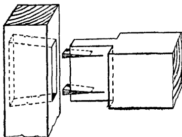
Fig. 158.—Method of Fox-wedging.
