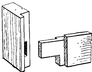
Fig 143.—Long and Short Shouldered Tenon.
