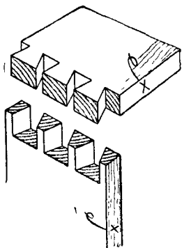
Fig. 310.—Through Dovetailing.
