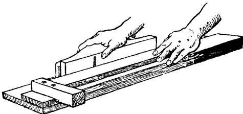
Fig. 26.—Method of using Shooting Board.
