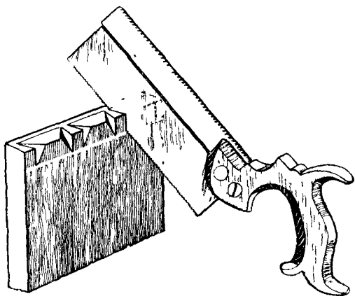
Fig. 274.—Removing the Waste Wood.
