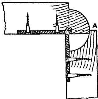
Fig. 252.—The Rule Joint with Leaf Down.
