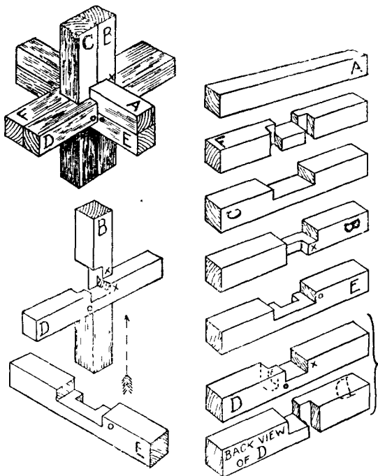
Fig. 388.—Six-piece Joint Puzzle.
