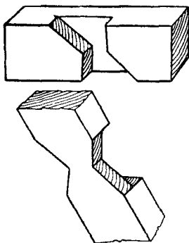
Fig. 54.—Carpentry Tie Joint.
