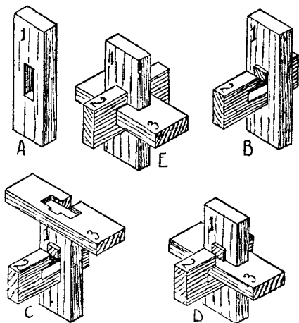
Fig. 389.—Mortising Puzzle, showing how the Parts Fit.
