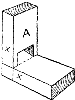
Fig. 305.—Testing.
