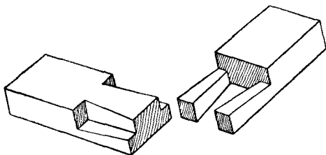
Fig. 42.—Dovetailed Halving Joint used for Lengthening Timber.
