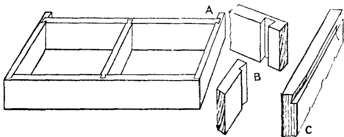
Fig. 284.—Constructional Frame (as for Plinth or Cornice) showing application of the Dovetail Joint.
