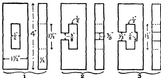
Fig. 390.—The Three Parts, with Sizes marked.
