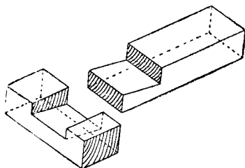
Fig. 41.—Tee Halving Joint.
