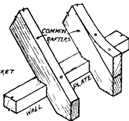
BIRDSMOUTH JOINTS AT SPARS AND WALL PLATES
