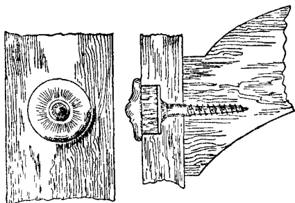
Fig. 358.—Patera Covers to Hide Screws.
