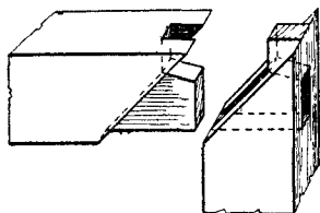
Fig. 146.—Self-wedging Japanese Tenon Joint.
