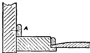
Fig. 253.—Shutting Stile of Cupboard Door.
