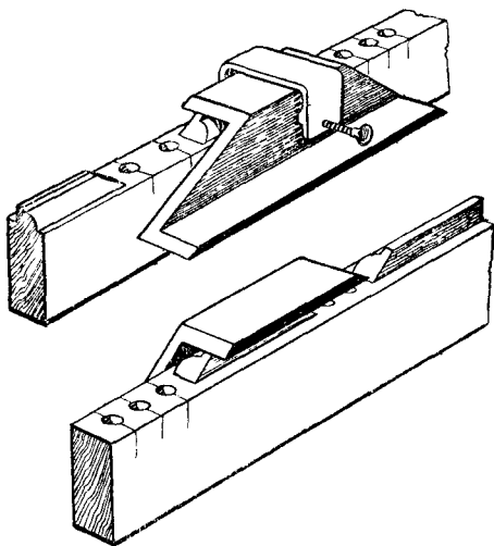
Fig. 333.—Template for Mitreing.
