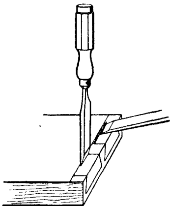
Fig. 311.—Chipping Waste of Lap Dovetail.
