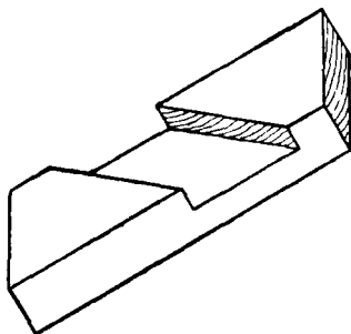
Figs. 49 and 50.—Separate pieces of Halved Moulded Joint.
