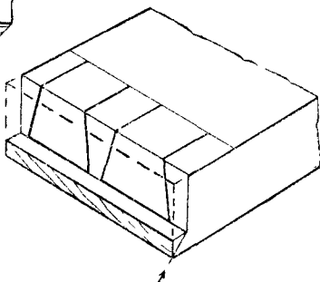
Fig. 286.—Housed and Mitred Dovetail.
