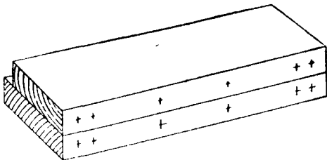
Fig. 198.—Marking and Gauging Boards for Dowelling.
