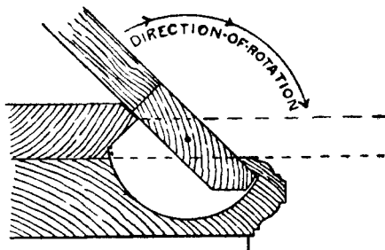
Fig. 242.—Fall Front of Writing Bureau.
