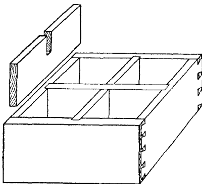
Fig. 59.—Cellarette Partition Joints.
