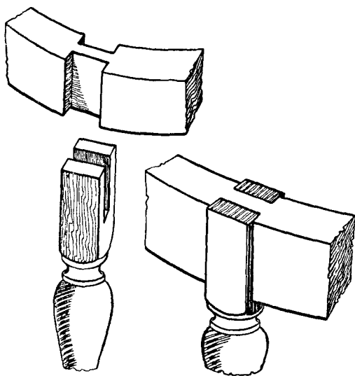
Fig. 73.—Table Leg Bridle-jointed to Rail.
