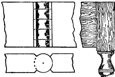
Fig. 246.—The Knuckle Joint Hinge.
