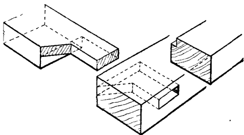
Fig. 142.—Haunched Tenon for Skylight or Garden Frame.
