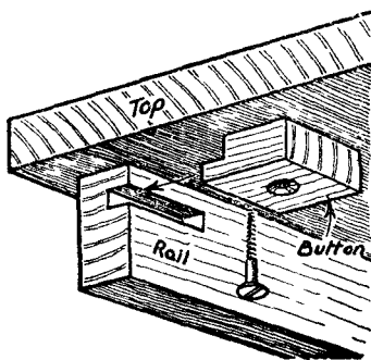
Fig. 359.—Method of Buttoning a Table Top.
