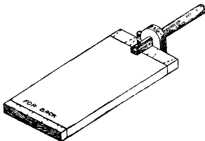
Fig. 273.—Method of Marking with Cutting Gauge.
