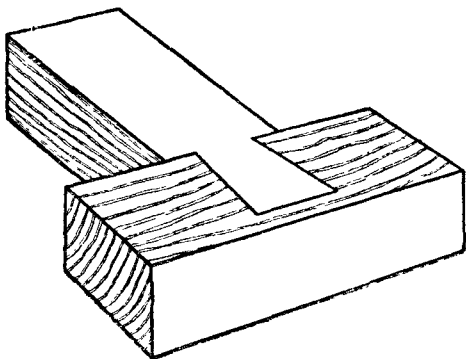
Fig. 401.—Blind Dovetail Puzzle Joint (see page 199).
