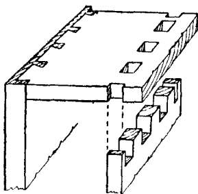
Fig 150.—Method of Pinning.
