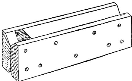
Fig. 191.—Cradle for Planing Dowels.
