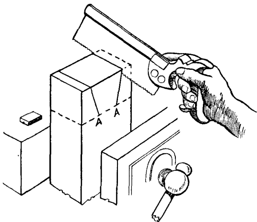
Fig. 308.—Sawing the Dovetails.
