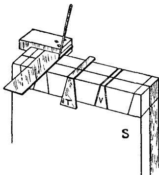
Fig. 272.—Squaring and use of Template.
