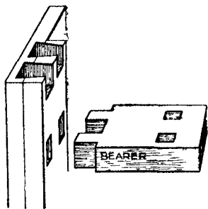
Fig. 149.—Twin Tenons.
