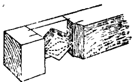
Fig. 185.—Mortise with Side Removed.
