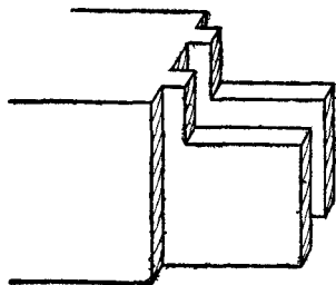
Fig. 168.—Twin Tenons for Thick Timber.
