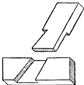
Fig. 37.—Oblique Dovetail Halving.
