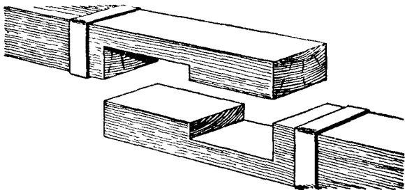
Fig. 219.—Example of Tabled Joint with Straps.
