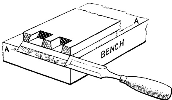
Fig. 287.—Working a Housed and Mitred Dovetail Joint.
