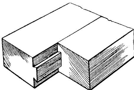
Fig. 102.—Joint with Single Dovetail Tongue and Groove.
