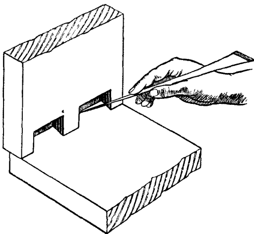
Fig. 307.—Marking Dovetails with Marking Awl.
