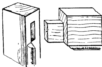
Fig. 148.—Mitred and Moulded Tenon Joint.
