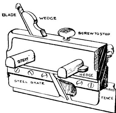
Fig. 121.—The Plough Plane and its Parts.
