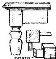
Fig. 167.—Detail of Table Framing.
