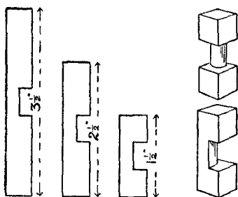
Fig. 370. Fig. 371. Fig. 372. Fig. 373. The Three Cross Pieces. Key Piece.
