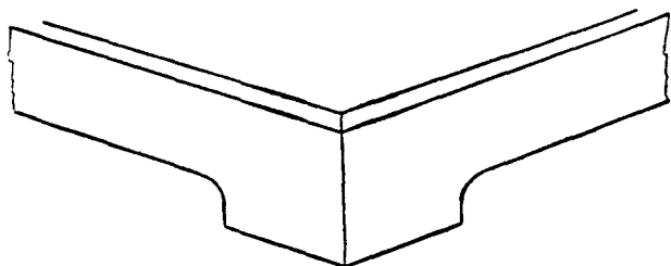
Fig. 15.—Butting Mitred Angle Joint.
