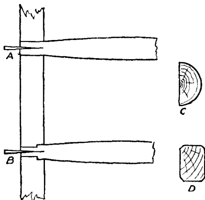
Fig. 344.—Ladder Rungs.
