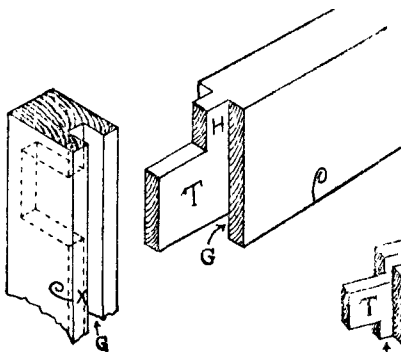
Fig. 187.—Removal of Haunching.
