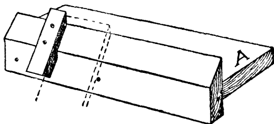
Fig. 327.—" Donkey's Ear " Shooting Board.
