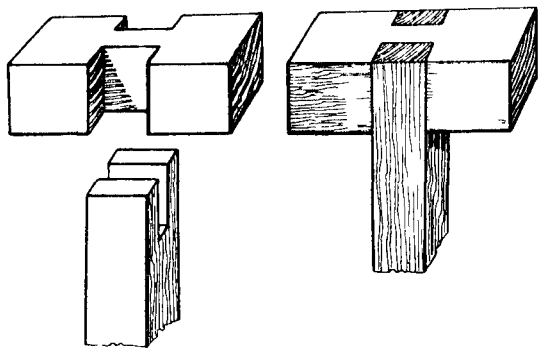
Fig. 72.—Simple Bridle Joint.
