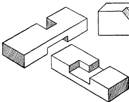
Fig. 52.—Manual Training Halved Exercise Joint.
