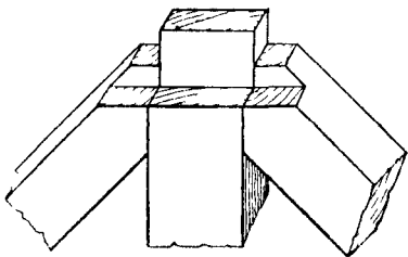
Fig. 138.—Joint used for Garden Gates.
