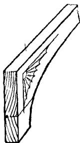
Fig. 20.— Jointing a shaped Spandrel.
