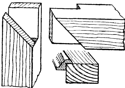
Fig. 159.—Tenon Joint with Mitred Face.
