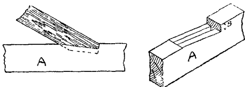
Fig. 356.—Rafter and Tie Beam Joint.
