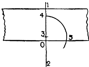
Fig. 251.—Setting Out for Rule Joint Hinge.
