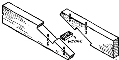
Fig. 218.—Detail of Scarfed Joint in Purlins.
