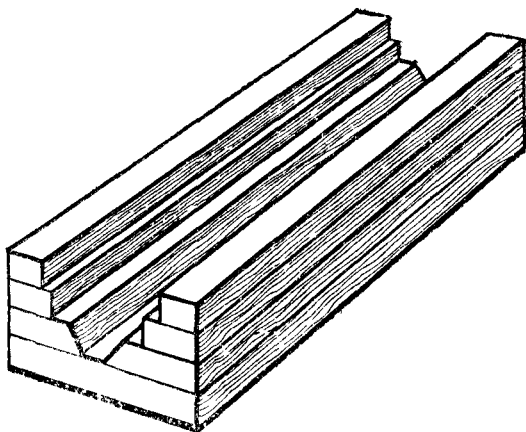
Fig. 342.—Half of Laminated Core Box.
