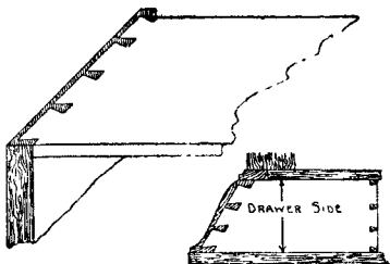
Fig. 294.—Lap-Dovetailing.
