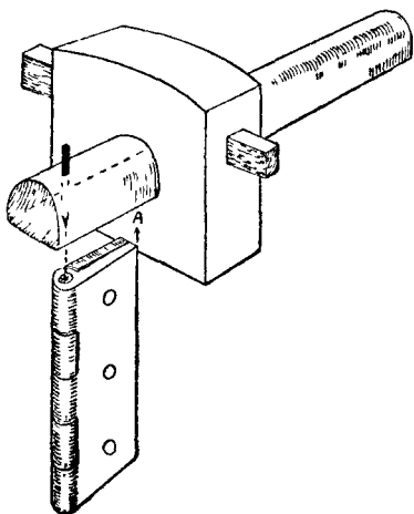
Fig. 223.—Gauging.
