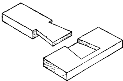
Fig. 38.—Stopped Dovetail Halving.
