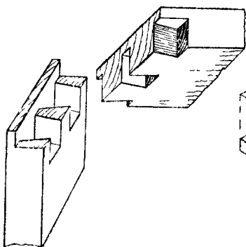
Fig. 285.—Blind Lap-Dovetailing.
