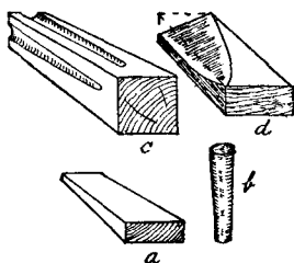
Fig. 364.—Wall Plugs, Four Varieties.
