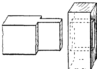
Fig. 134.—Joint for Inside Framing.
