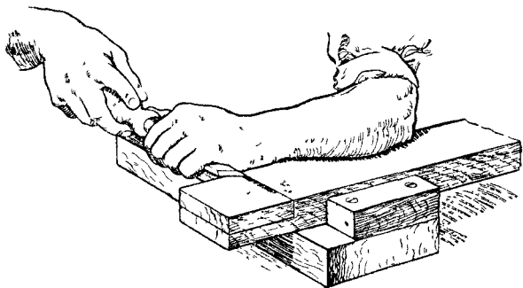
Fig. 66.—Chiselling away Wood up to Gauge Line.
