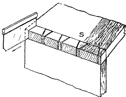
Fig. 279.—Marking by means of Saw Blade.
