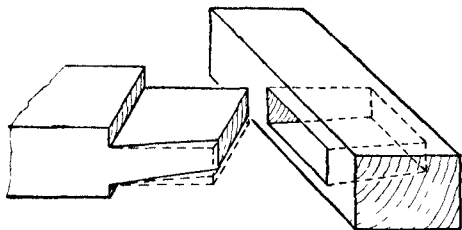
Fig. 156.—Wheelwright's Self-wedging Tenon Joint.
