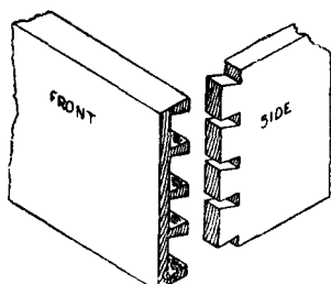
Fig. 270.—Lap-dovetailing for Drawers.
