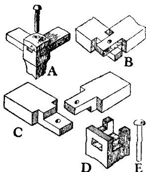
Fig. 348.—Joint for Home-made Cot.
