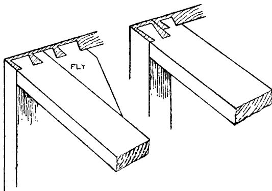
Fig. 293.—Carcass Work, showing Bearer Rails Dovetailed.
