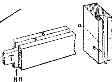
Fig. 188.—Haunching with Groove above.
