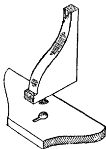
Fig. 366.—Slot Screwing a Bracket.
