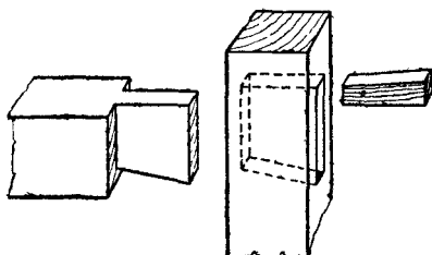
Fig. 157.—Dovetailed and Wedged Tenon.
