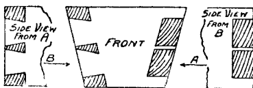
Fig. 298.—Oblique Dovetailing.
