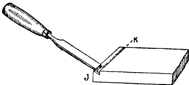
Fig. 320.—Channelling the Alternate Piece.
