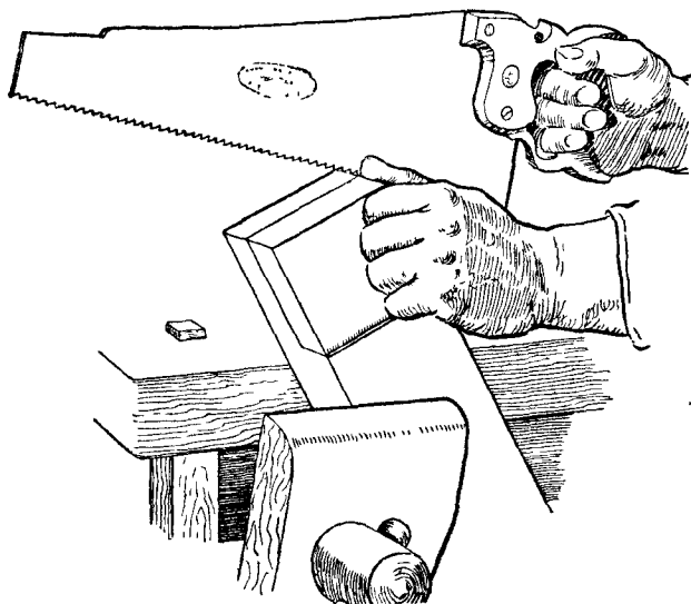
Fig. 70.—Sawing the Cheek of a Halving Joint.
