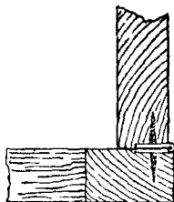
Fig. 241.—Section.
