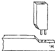
Fig. 206.—Dowelling for Moulded Frame.
