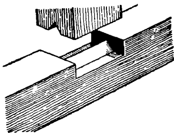
Fig. 351.—The Saddle Joint.
