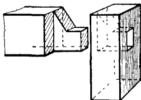
Fig. 135.—Haunched Barefaced Tenon.
