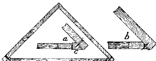
Fig. 237.—Hinging Door of Corner Cupboard.
