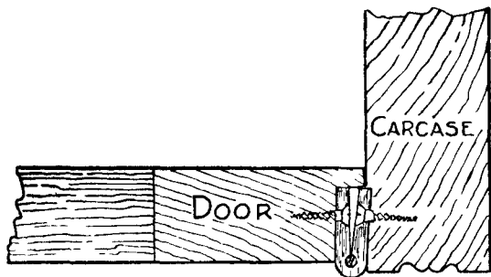
Fig. 238.—Inside Hinging : Method of Letting Butt Hinge into Door Frame and Carcase.
