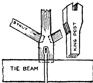
Fig. 161.—Roof Joints.
