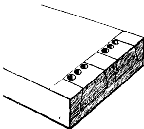
Fig. 277.—Roughing-out by Boring.
