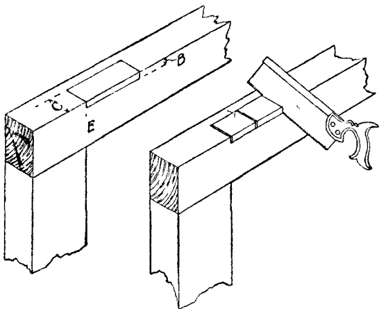
Fig. 225.—Sawing for the Recess.
