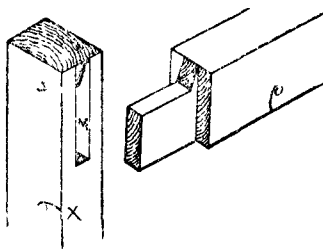
Fig. 186.—The Joint Separated.
