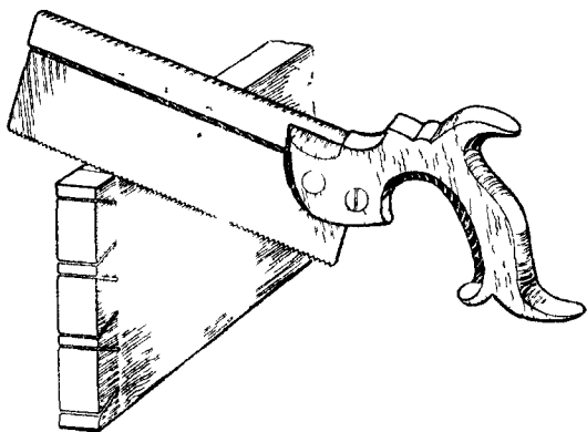
Fig. 275.—Cutting away the Half Dovetails.
