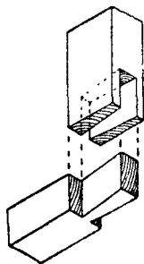
Fig. 267.—A Single Through Dovetail.
