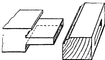
Fig. 147.—Tenoned and Scribed Joint.
