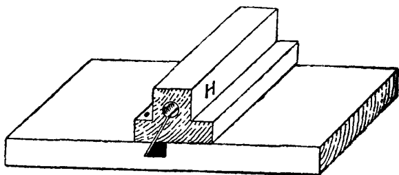
Fig. 318.—Guide Block for Bevelling.
