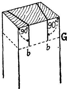
Fig. 303.—Marking the Pins.
