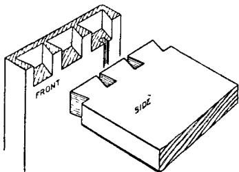
Fig. 309.—Lap-dovetailing Drawer Front to Drawer Side.
