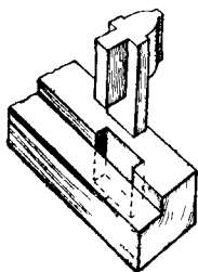
Fig. 165.—Tenoning Moulded Sash Bar.
