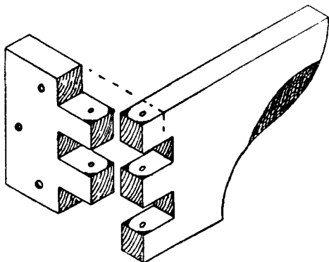
Fig. 245.—Finger Joint Hinge.
