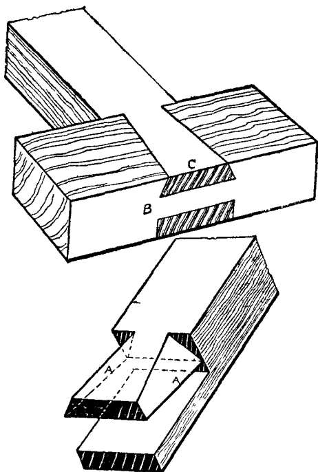
Fig. 386.—Variation of the Dovetail Puzzle.
