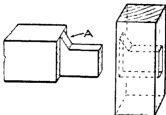
Fig. 130.—Haunched Tenon used at end of Door Frame.
