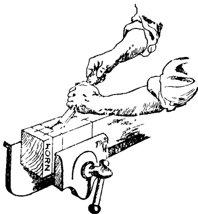
Fig. 184.—Removing Waste of Mortise with Chisel.
