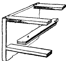
Fig. 108. —Part Carcase of Dressing Table.
